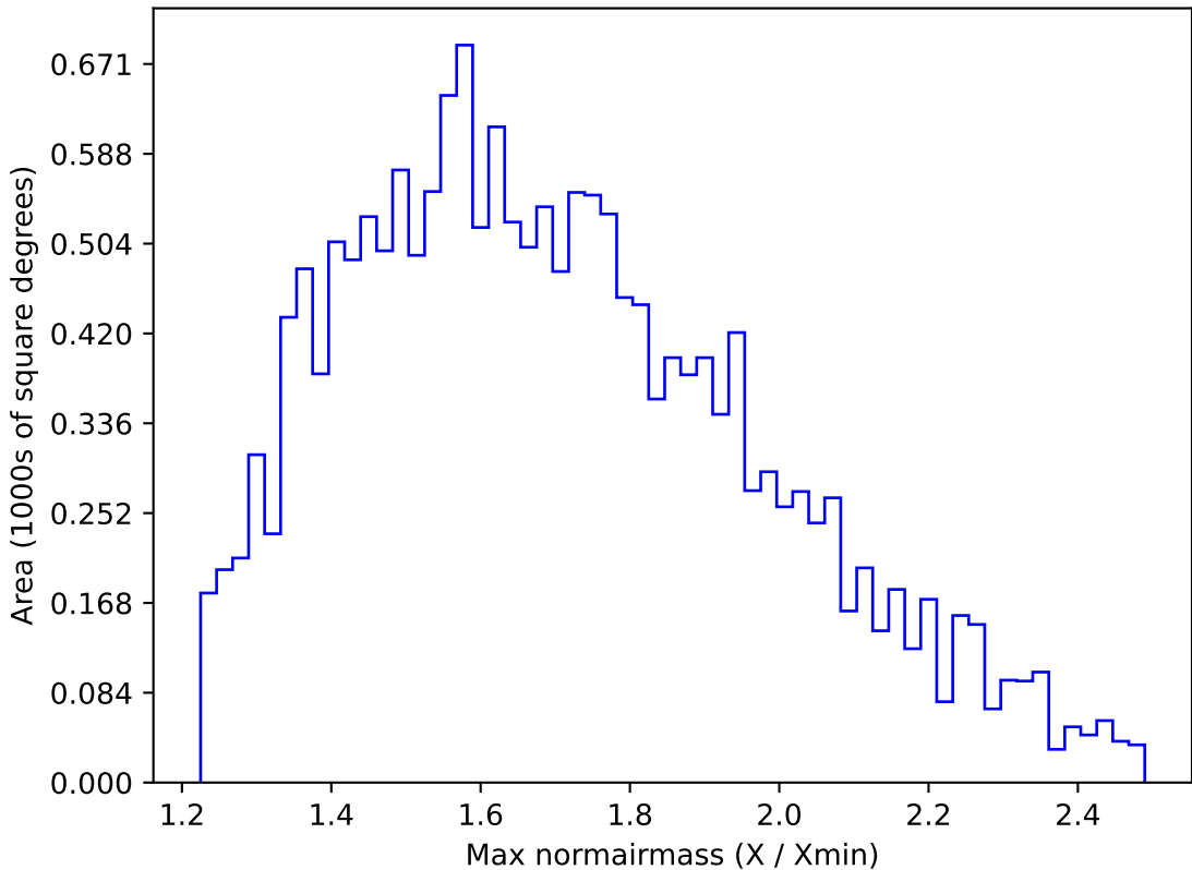
weather_cloudso8v3.4_10yrs WFD u band: Max normairmass
