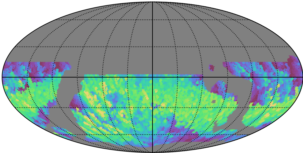
weather_cloudso8v3.4_10yrs WFD r band: Max normairmass
