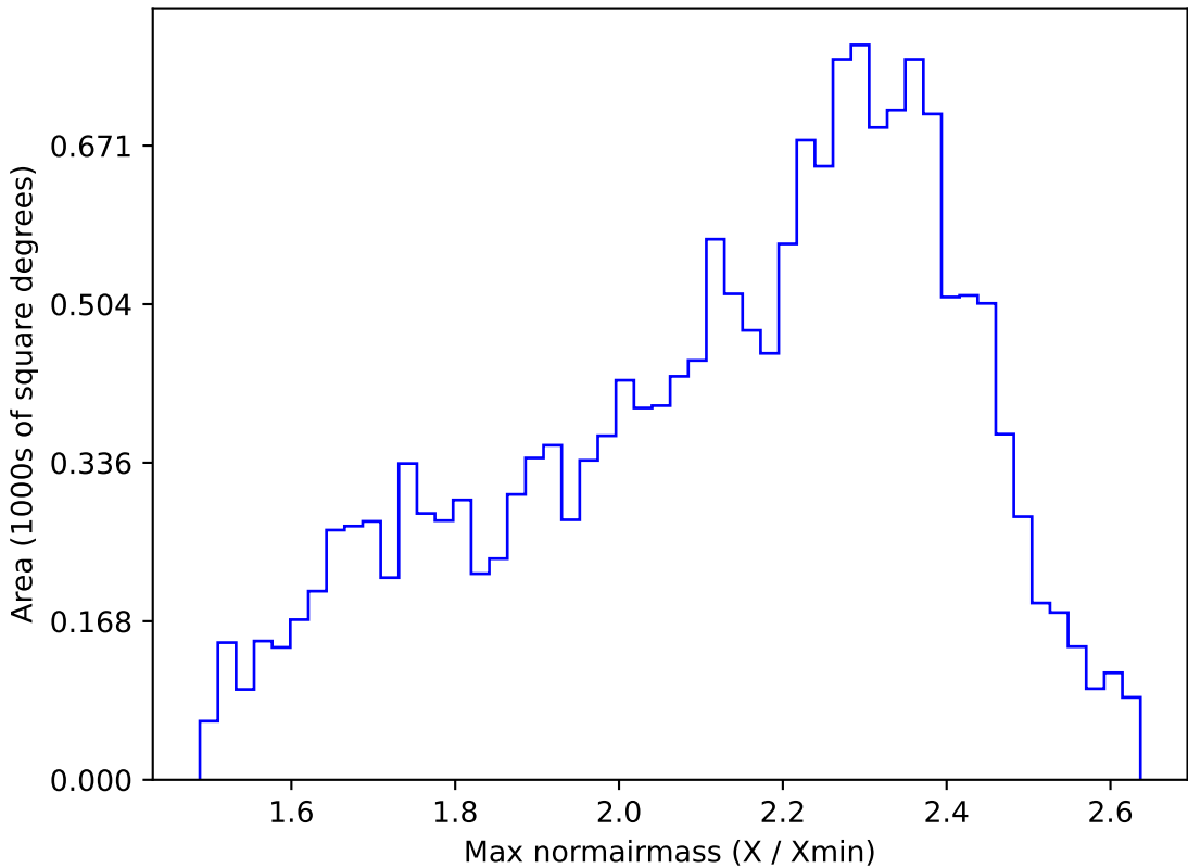
weather_cloudso8v3.4_10yrs WFD r band: Max normairmass
