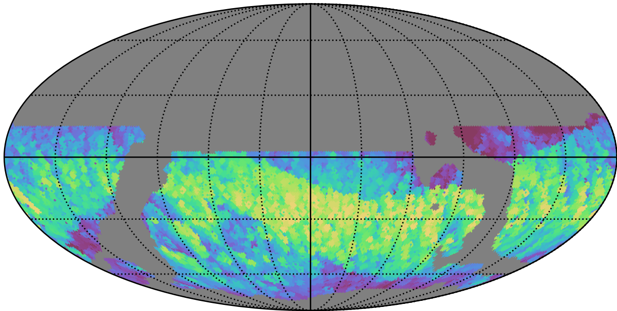
weather_cloudso8v3.4_10yrs WFD i band: Max normairmass
