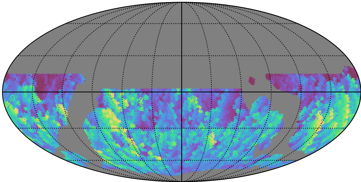
weather_cloudso8v3.4_10yrs WFD g band: Max normairmass
