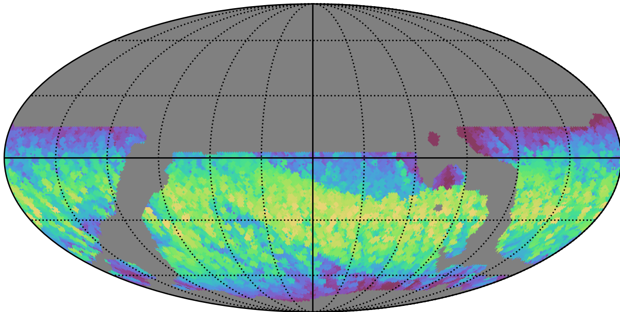
weather_cloudso8v3.4_10yrs WFD all bands: Max normairmass
