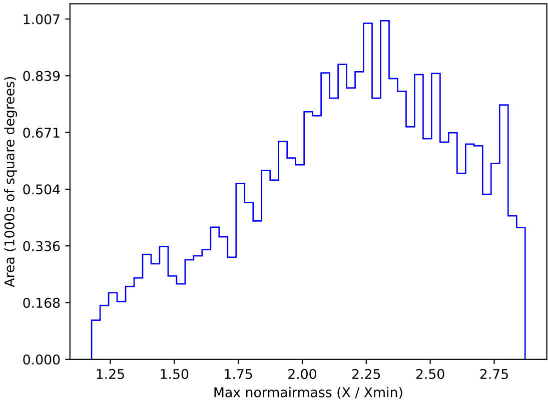
weather_cloudso8v3.4_10yrs All sky z band: Max normairmass
