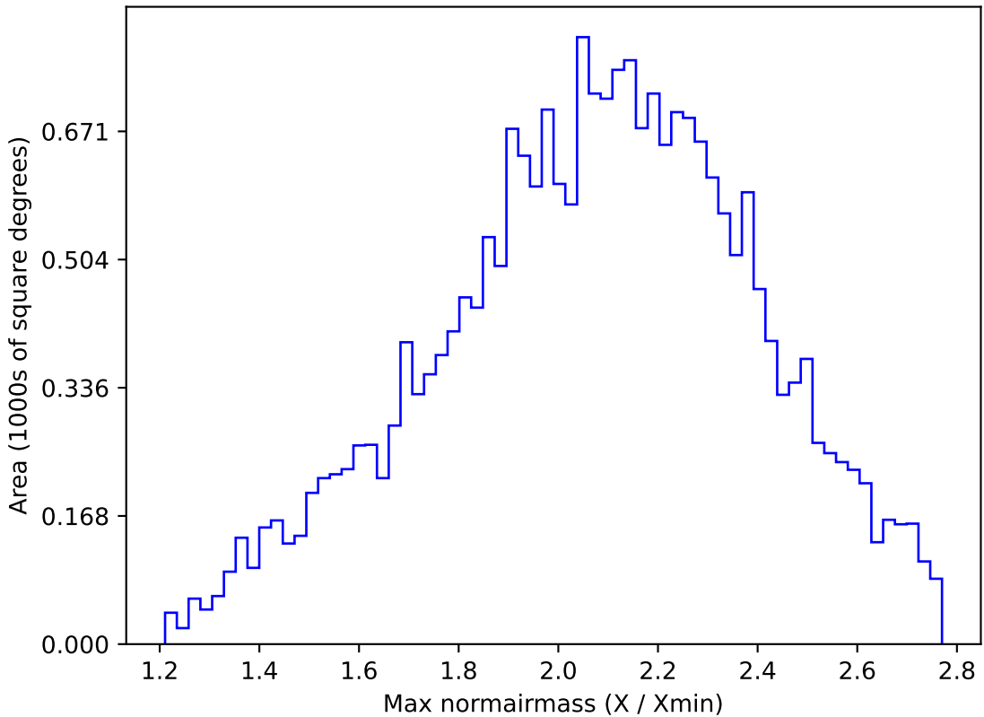
weather_cloudso8v3.4_10yrs All sky y band: Max normairmass
