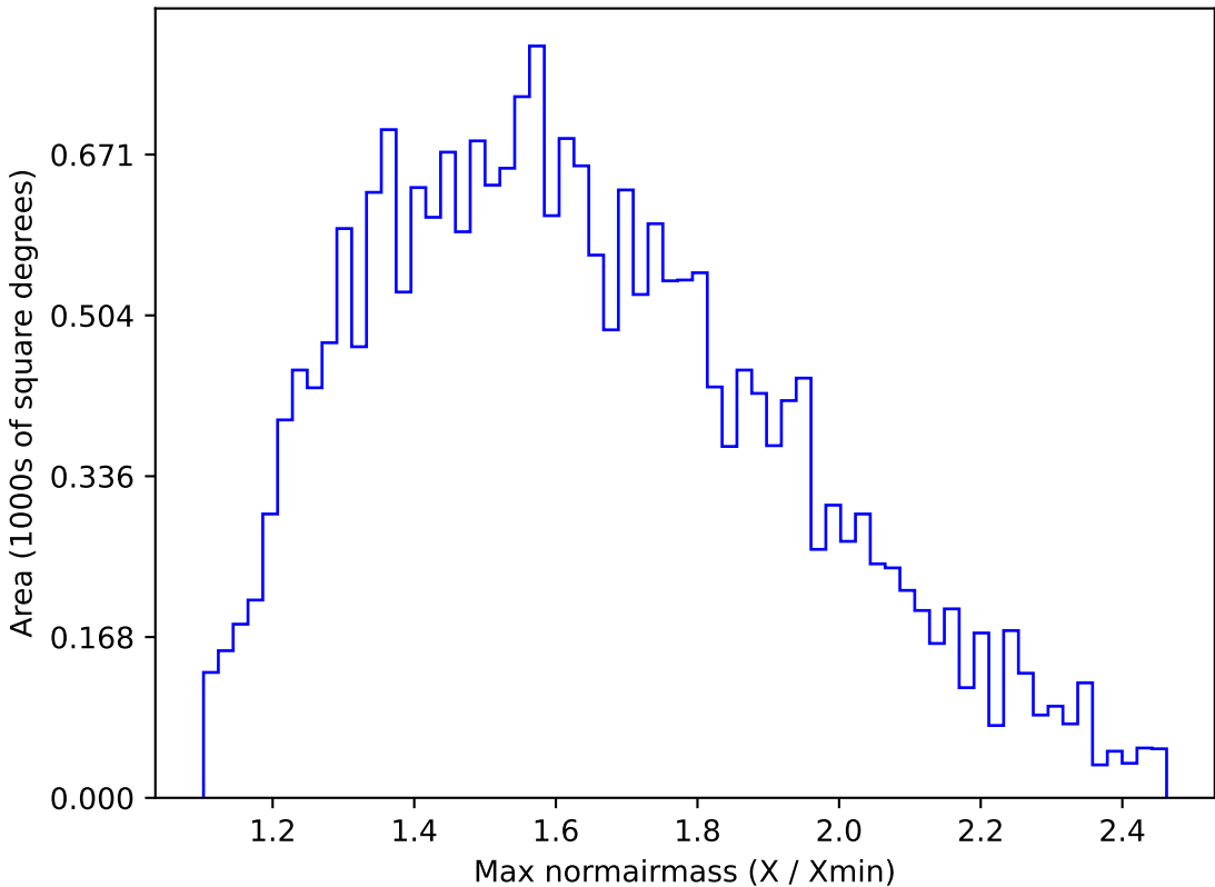
weather_cloudso8v3.4_10yrs All sky u band: Max normairmass
