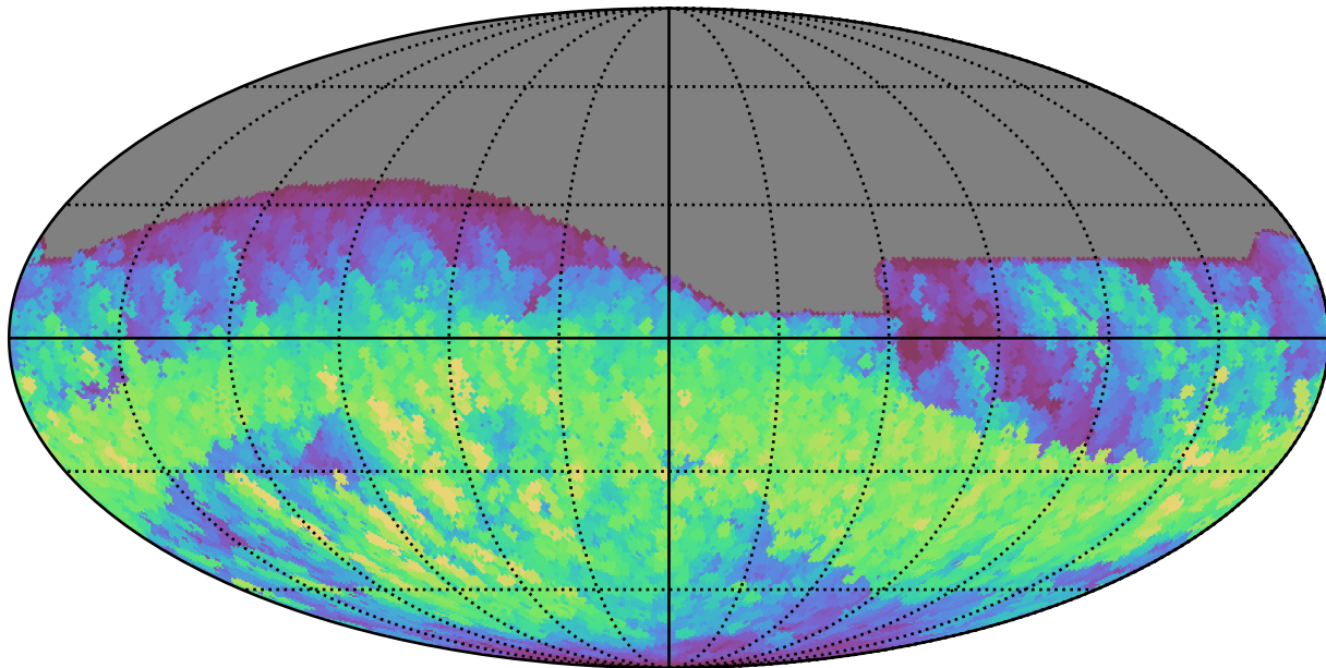
weather_cloudso8v3.4_10yrs All sky r band: Max normairmass
