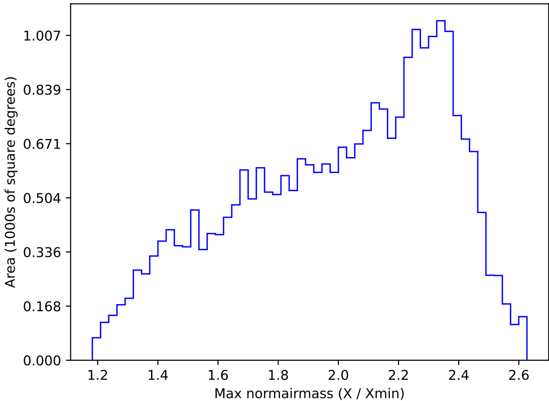
weather_cloudso8v3.4_10yrs All sky r band: Max normairmass
