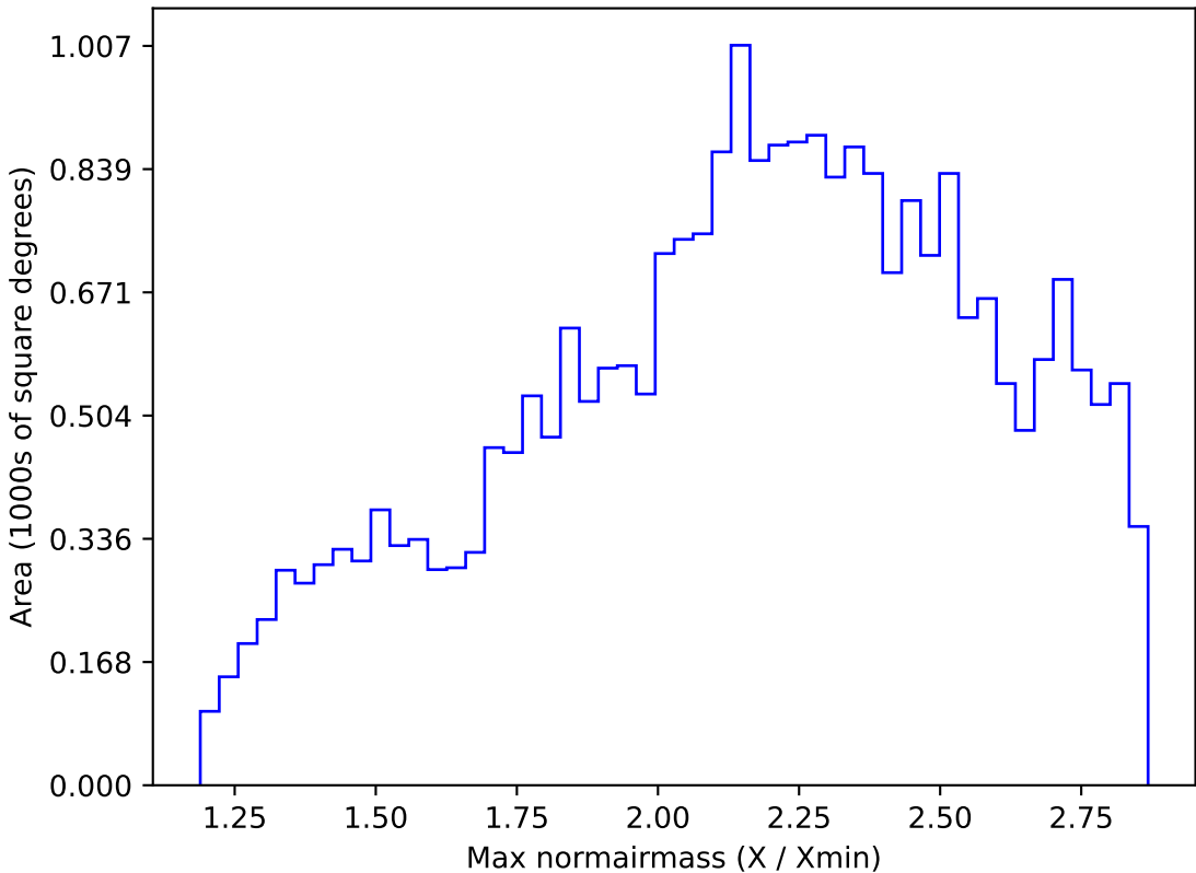
weather_cloudso8v3.4_10yrs All sky i band: Max normairmass
