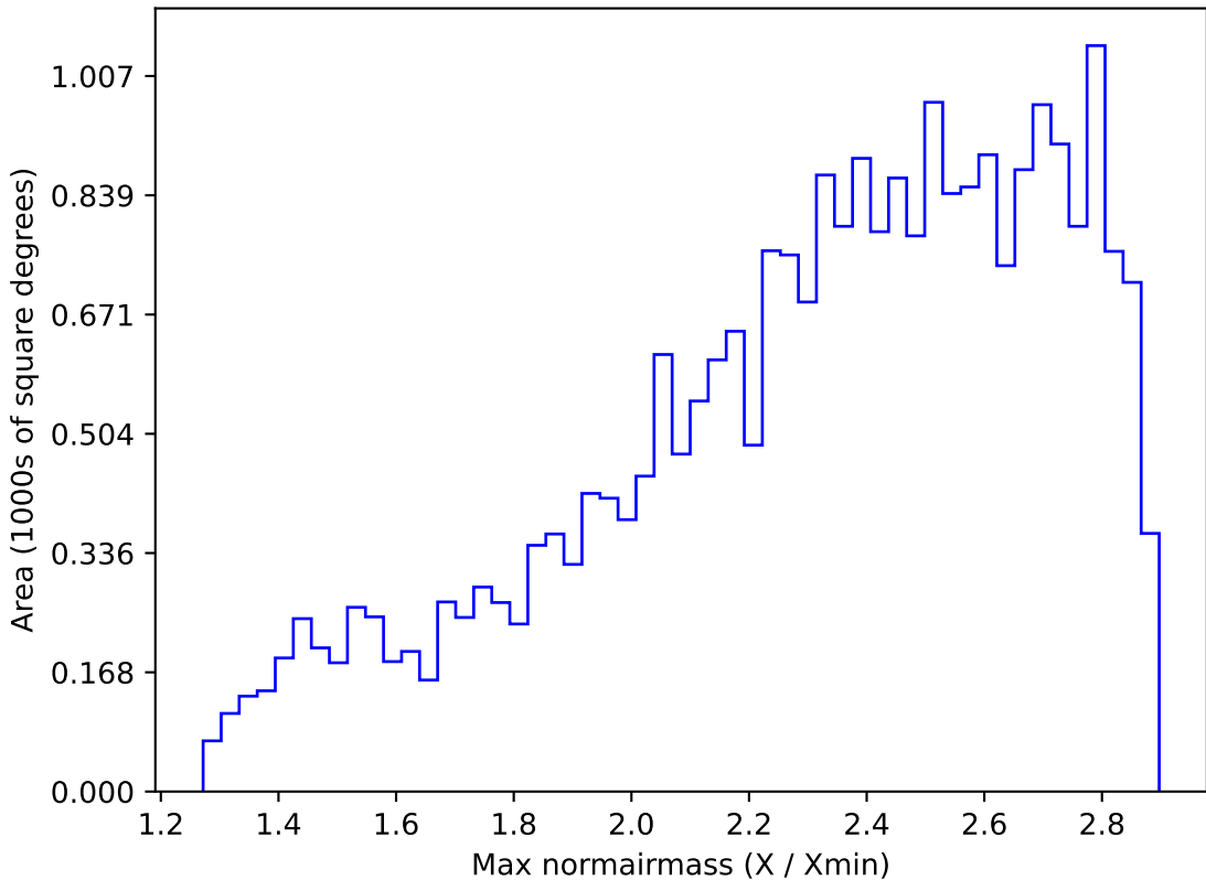
weather_cloudso8v3.4_10yrs All sky all bands: Max normairmass
