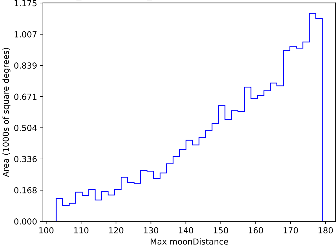
weather_cloudso8v3.4_10yrs WFD z band: Max moonDistance
