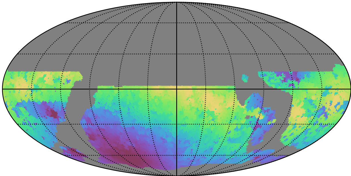
weather_cloudso8v3.4_10yrs WFD y band: Max moonDistance
