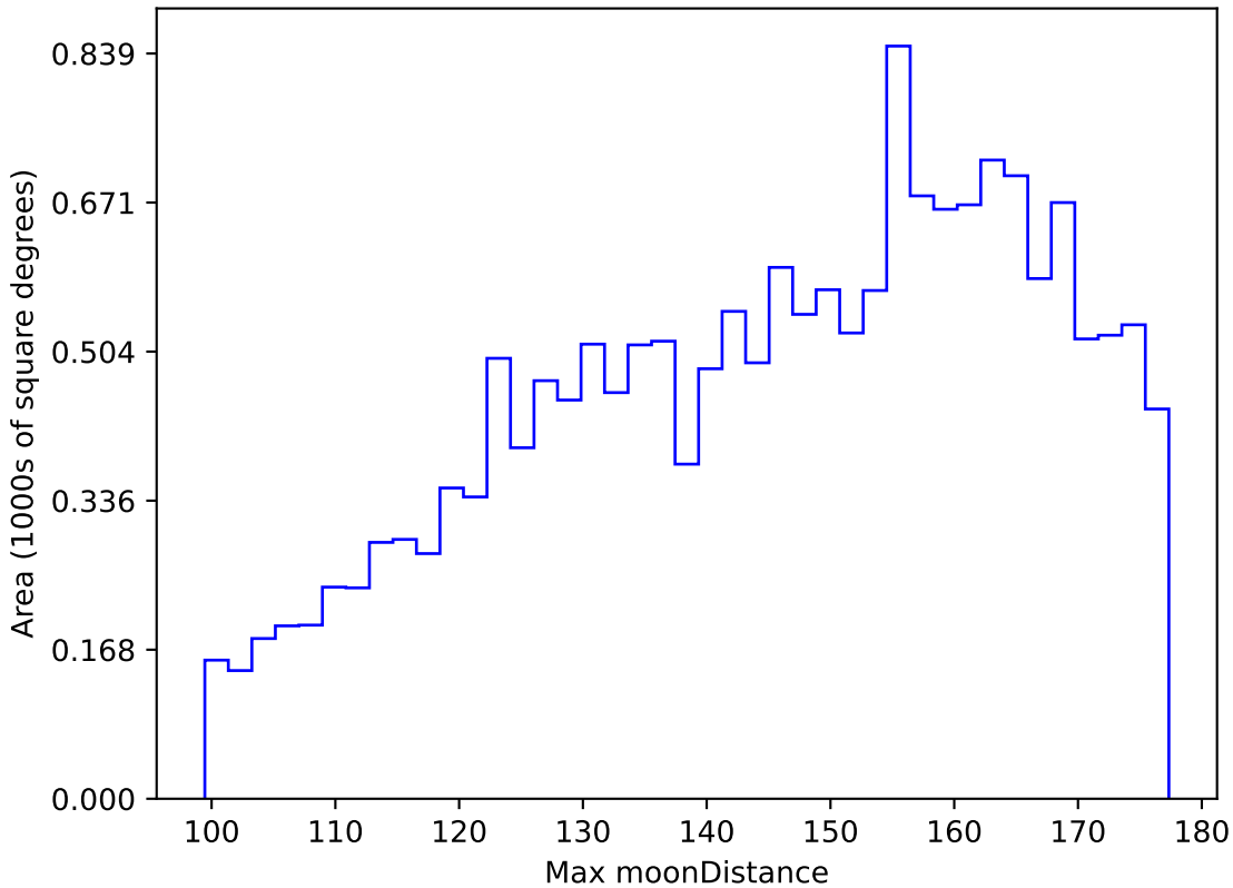
weather_cloudso8v3.4_10yrs WFD y band: Max moonDistance
