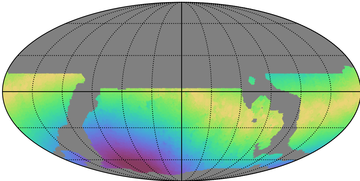
weather_cloudso8v3.4_10yrs WFD u band: Max moonDistance
