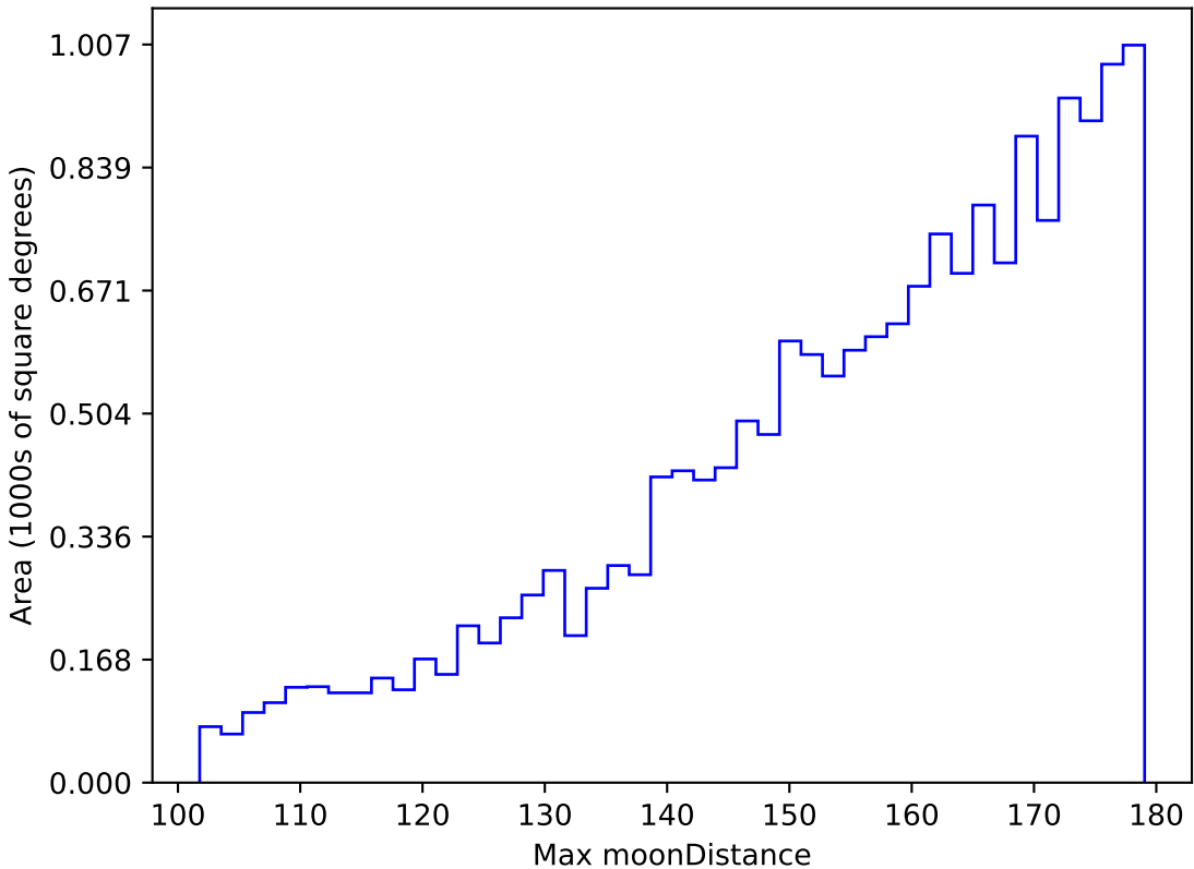
weather_cloudso8v3.4_10yrs WFD u band: Max moonDistance
