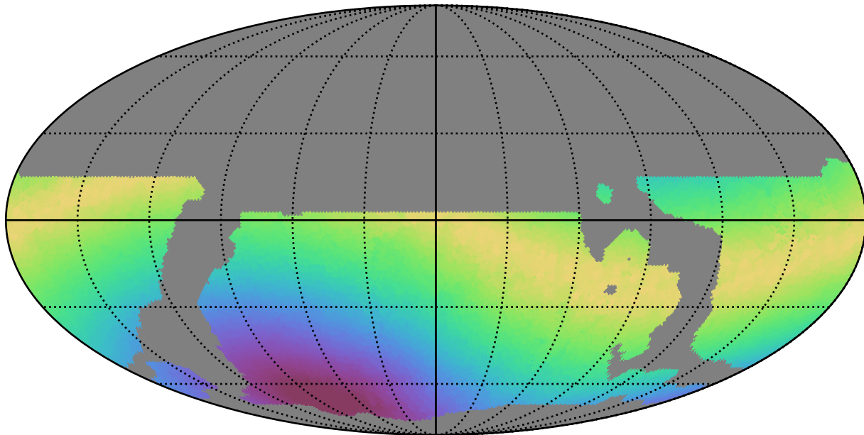
weather_cloudso8v3.4_10yrs WFD r band: Max moonDistance
