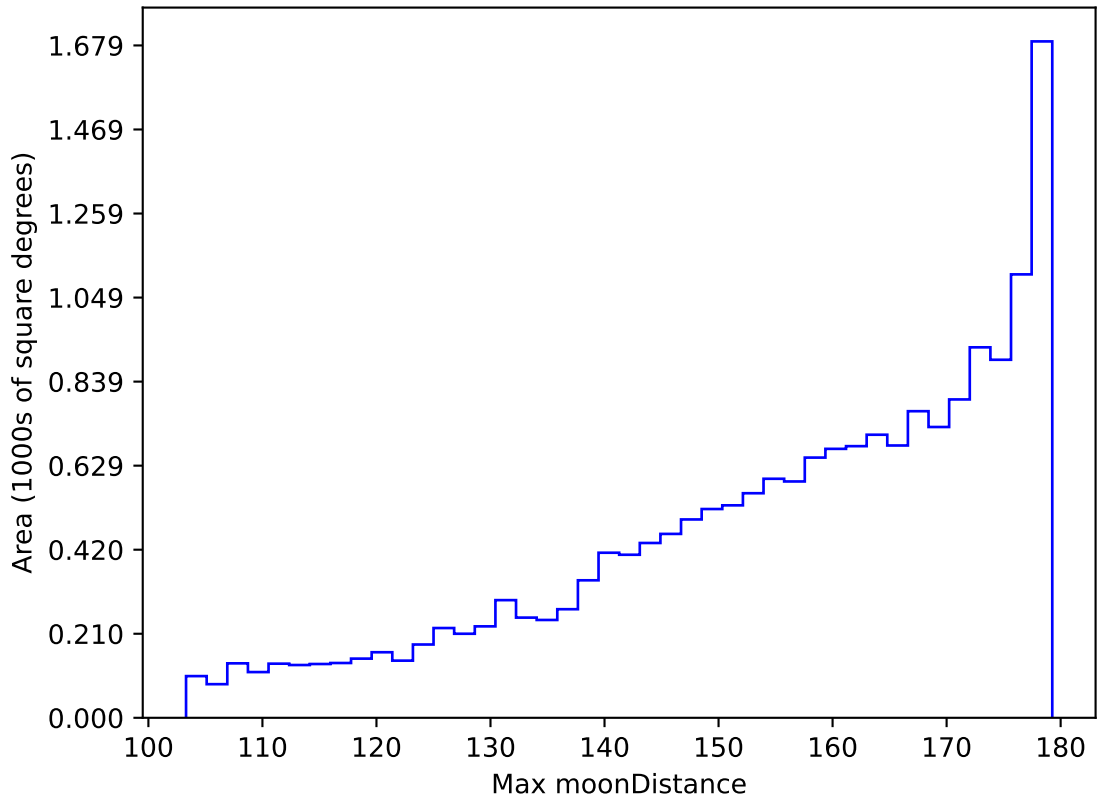
weather_cloudso8v3.4_10yrs WFD r band: Max moonDistance
