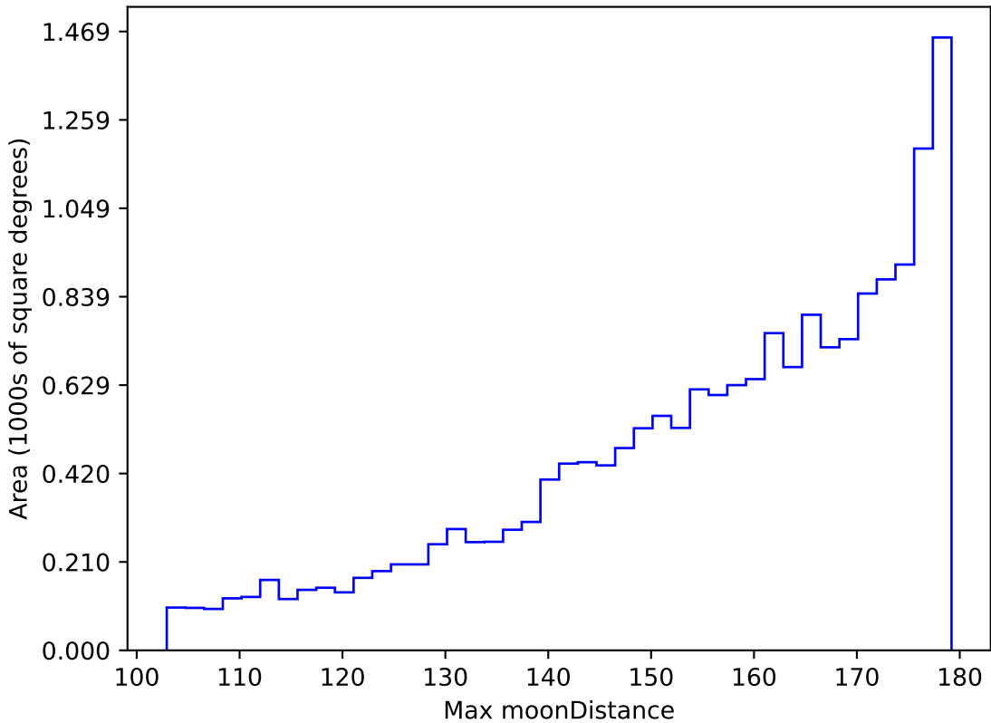
weather_cloudso8v3.4_10yrs WFD i band: Max moonDistance
