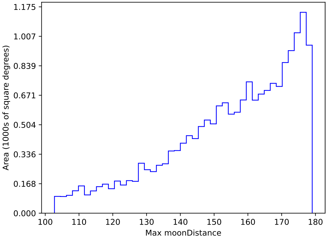
weather_cloudso8v3.4_10yrs WFD g band: Max moonDistance
