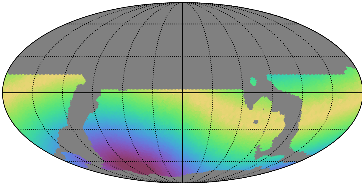
weather_cloudso8v3.4_10yrs WFD all bands: Max moonDistance
