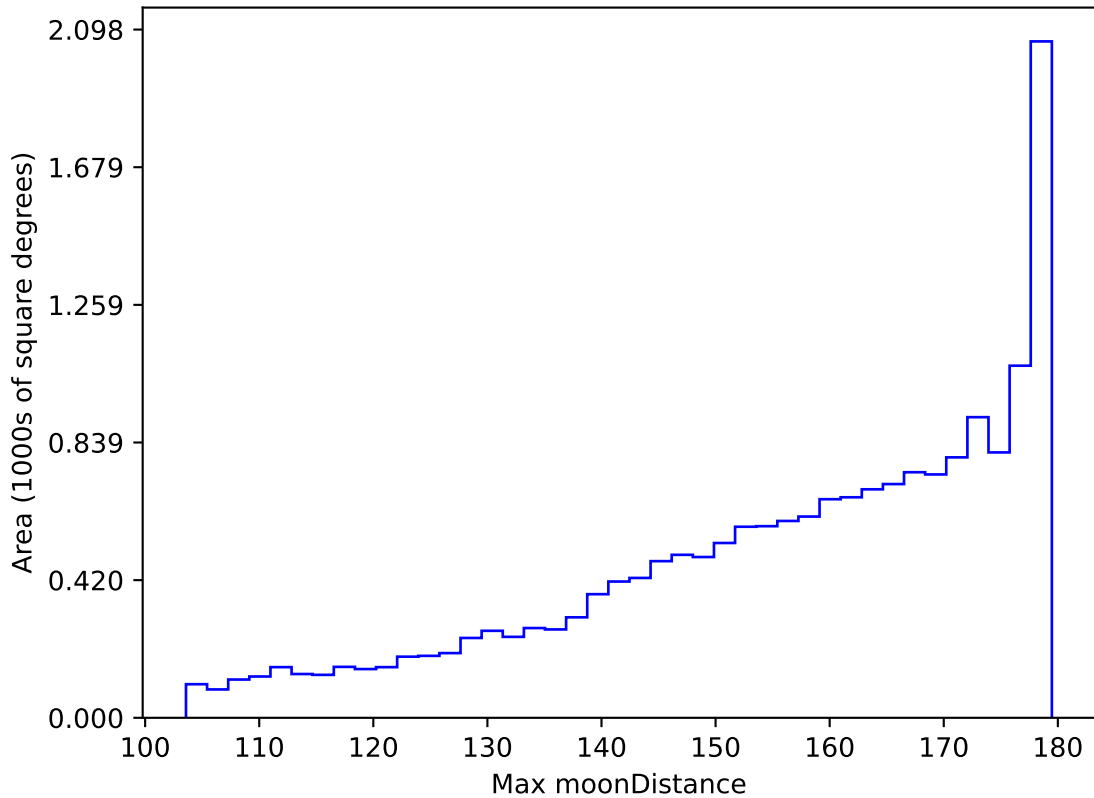
weather_cloudso8v3.4_10yrs WFD all bands: Max moonDistance
