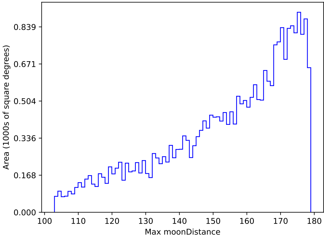
weather_cloudso8v3.4_10yrs All sky z band: Max moonDistance
