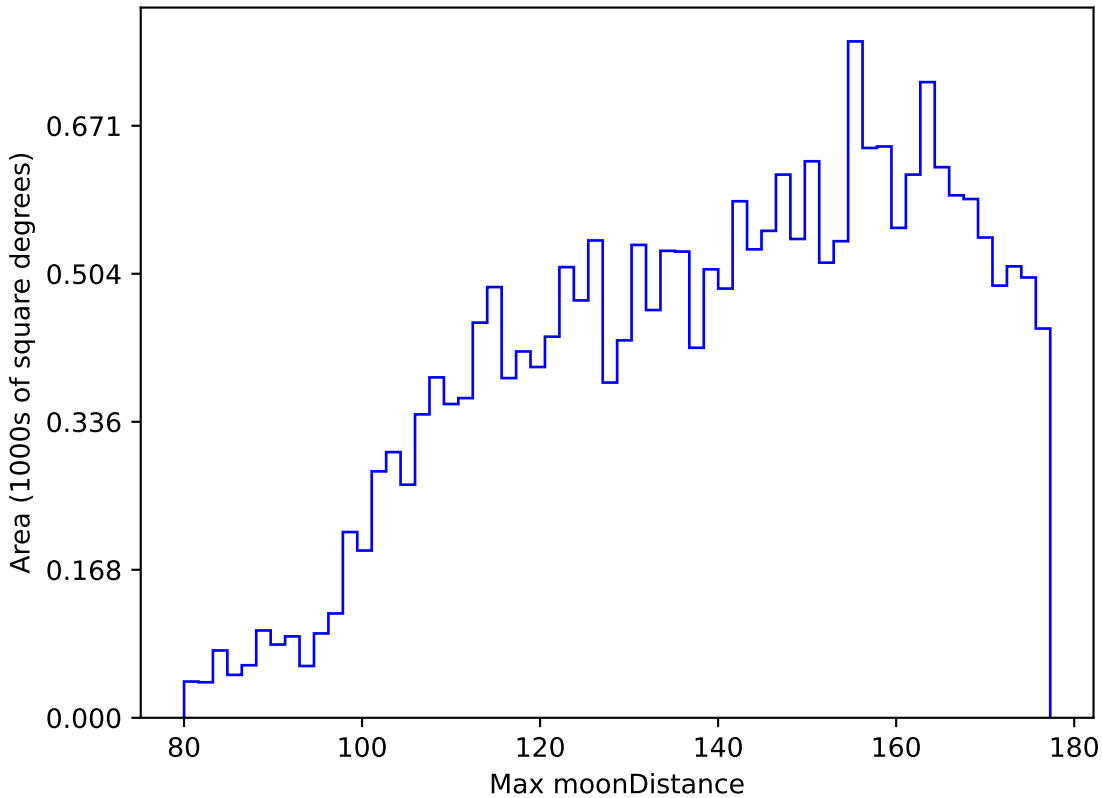
weather_cloudso8v3.4_10yrs All sky y band: Max moonDistance
