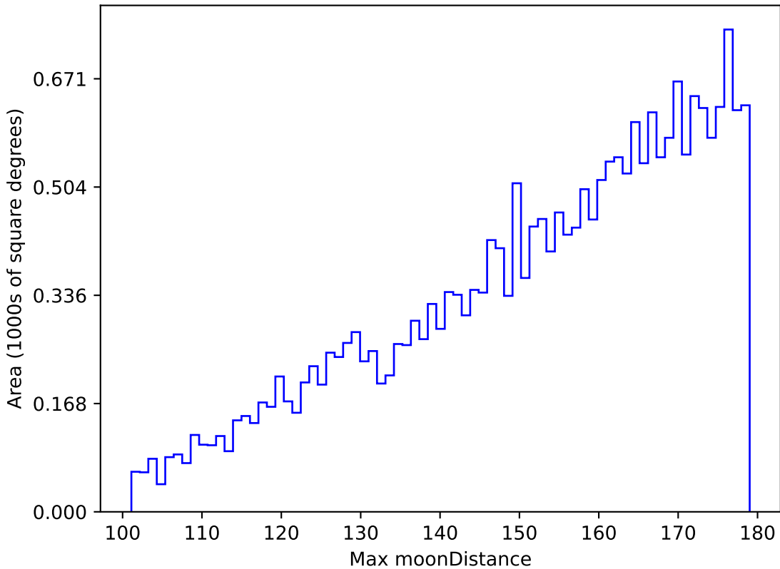
weather_cloudso8v3.4_10yrs All sky u band: Max moonDistance
