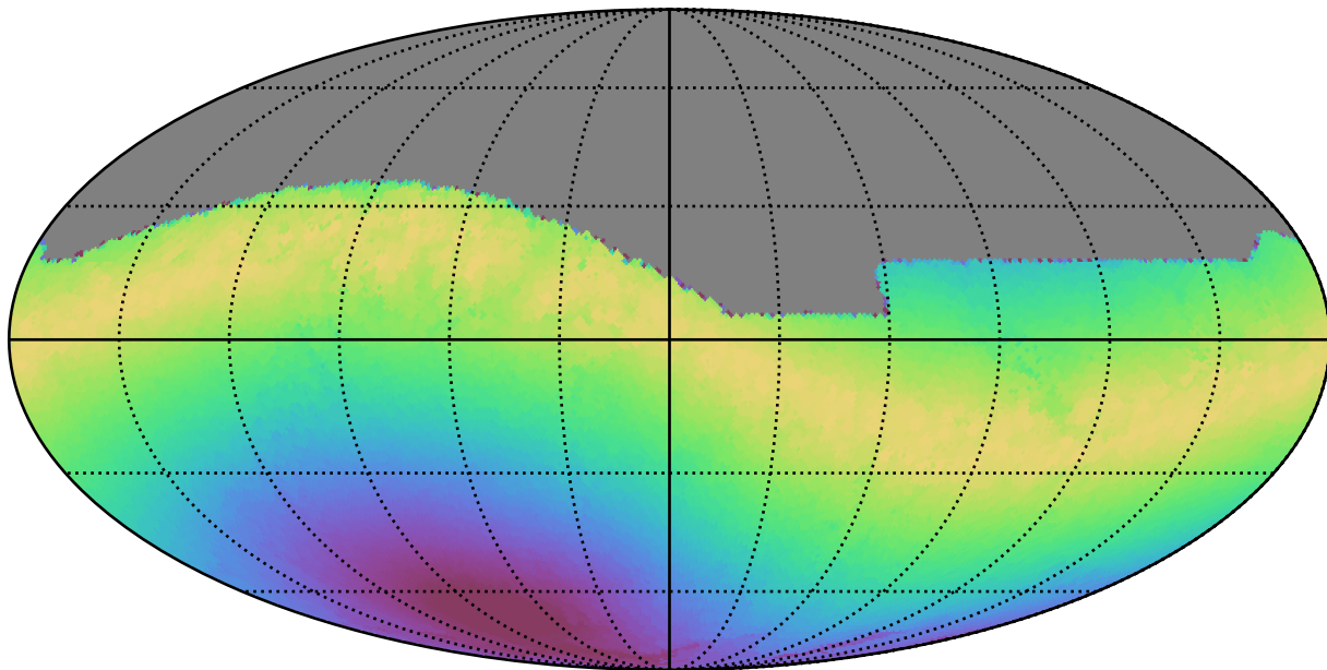
weather_cloudso8v3.4_10yrs All sky r band: Max moonDistance
