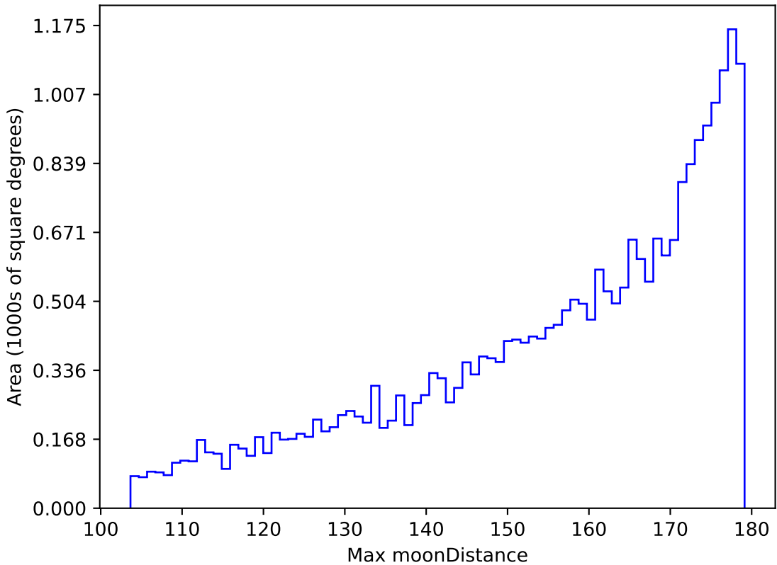
weather_cloudso8v3.4_10yrs All sky i band: Max moonDistance
