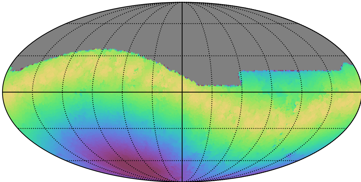
weather_cloudso8v3.4_10yrs All sky g band: Max moonDistance
