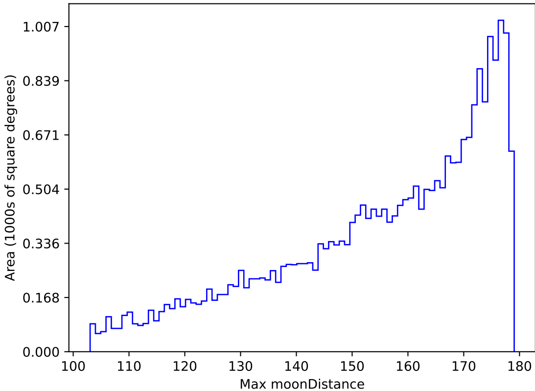
weather_cloudso8v3.4_10yrs All sky g band: Max moonDistance
