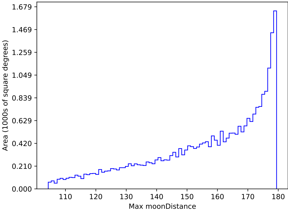
weather_cloudso8v3.4_10yrs All sky all bands: Max moonDistance
