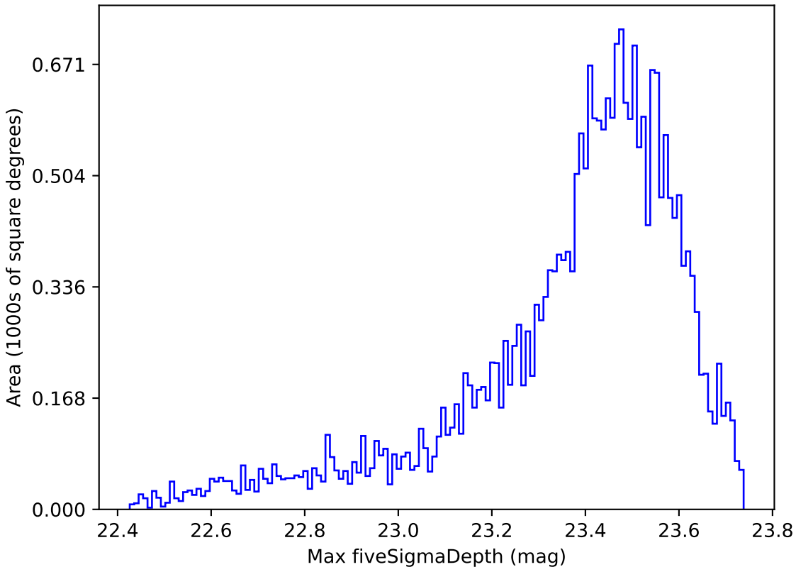
weather_cloudso8v3.4_10yrs Yr 1 z band: Max fiveSigmaDepth
