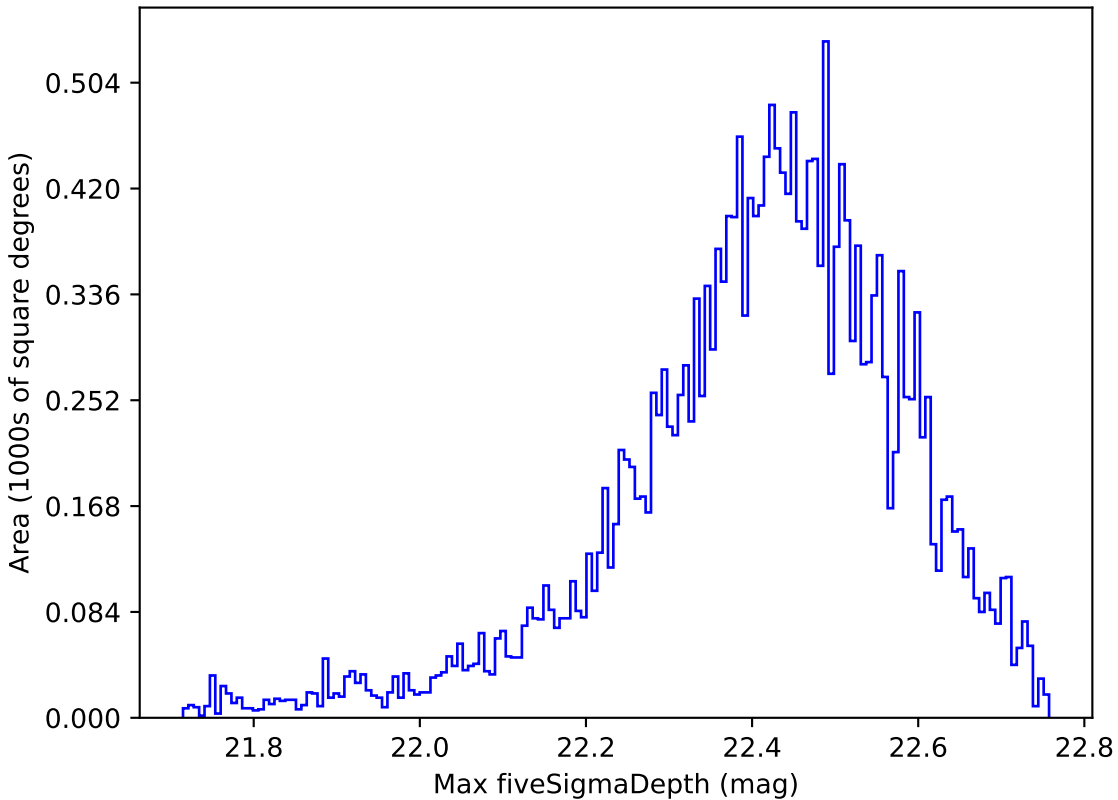
weather_cloudso8v3.4_10yrs Yr 1 y band: Max fiveSigmaDepth
