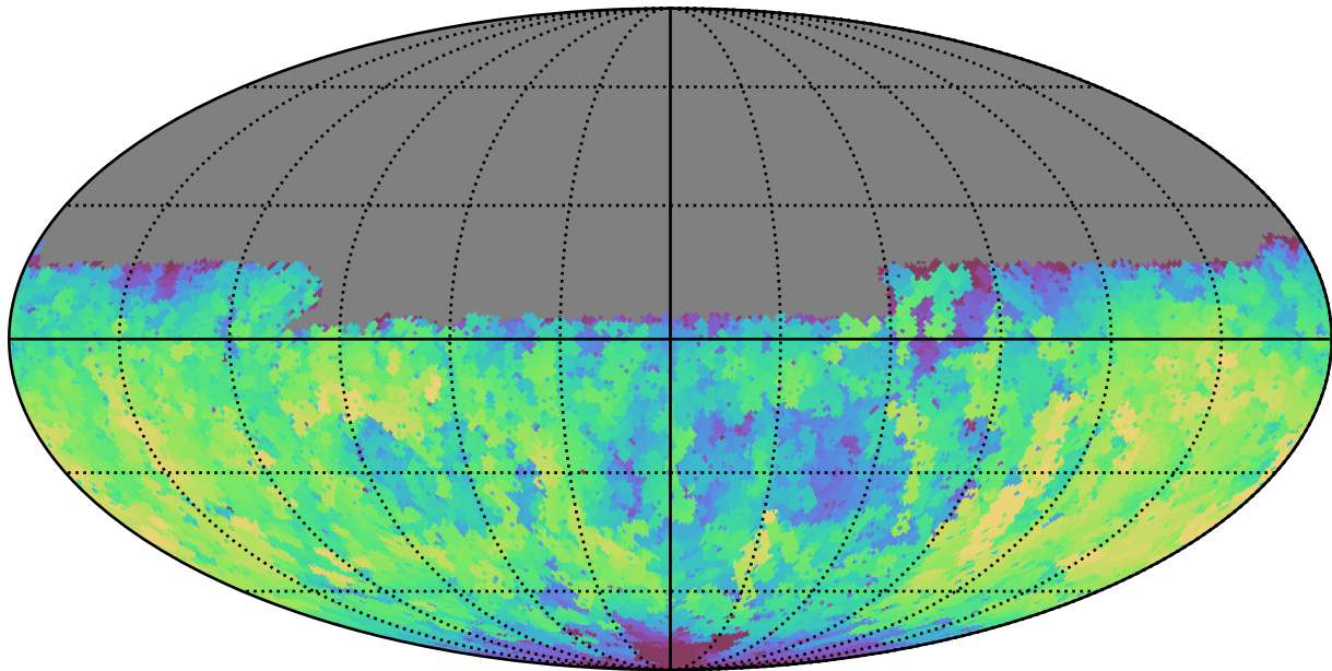
weather_cloudso8v3.4_10yrs Yr1 u band: Max fiveSigmaDepth
