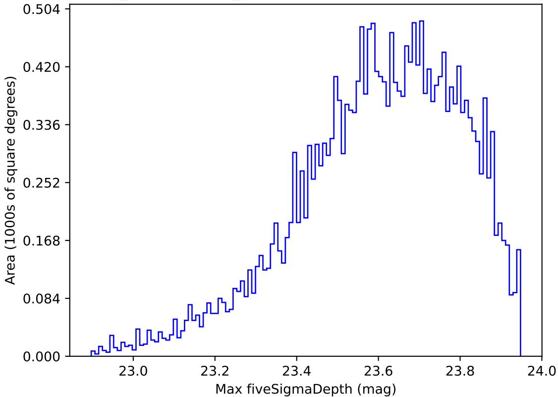
weather_cloudso8v3.4_10yrs Yr 1 u band: Max fiveSigmaDepth
