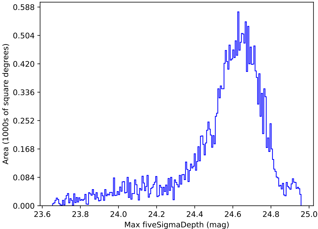
weather_cloudso8v3.4_10yrs Yr 1 r band: Max fiveSigmaDepth
