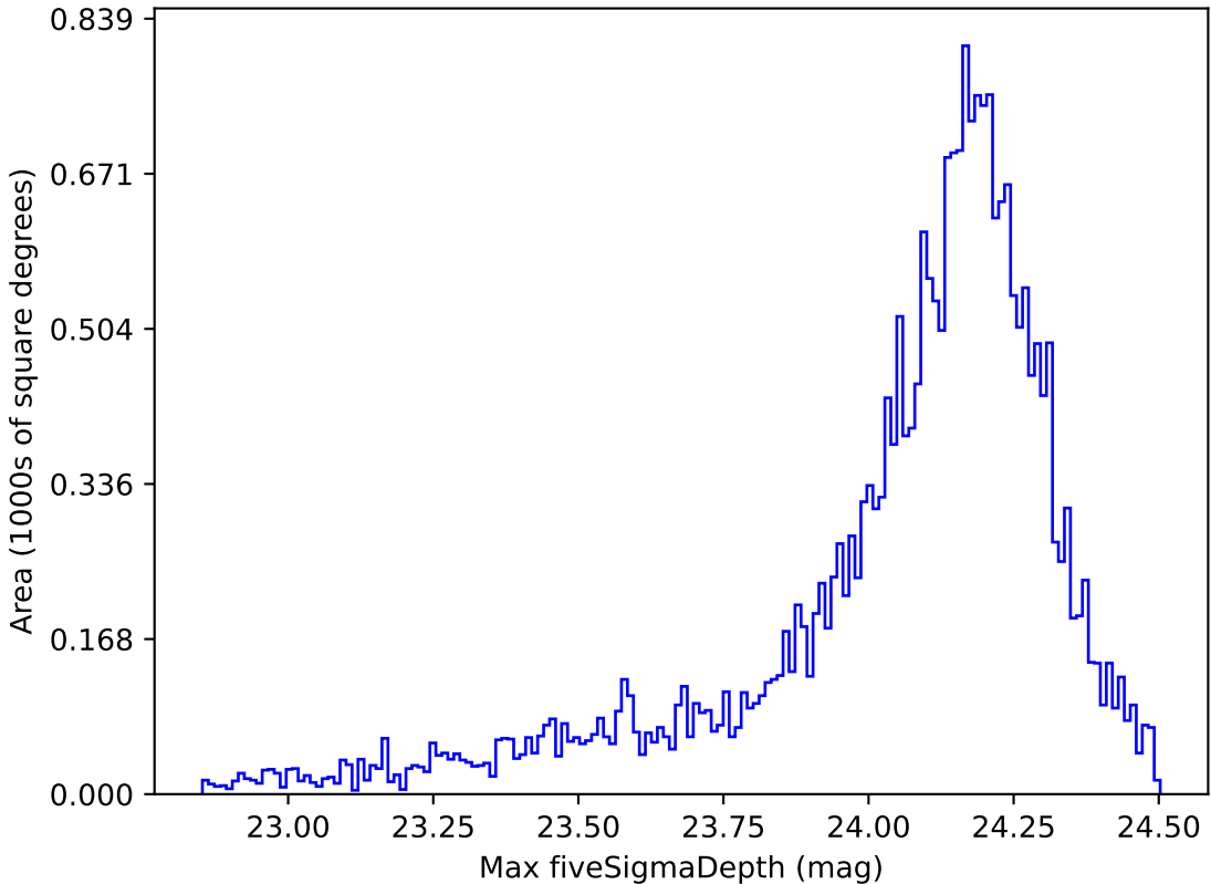
weather_cloudso8v3.4_10yrs Yr 1 i band: Max fiveSigmaDepth
