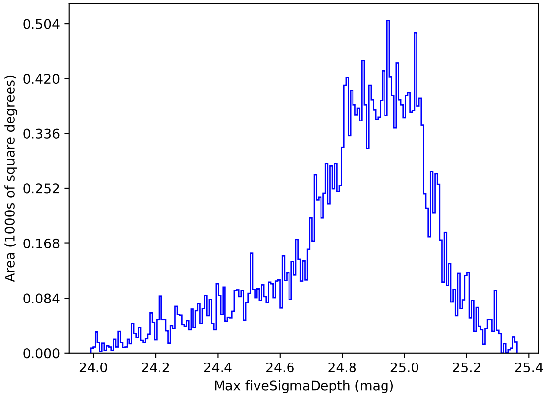
weather_cloudso8v3.4_10yrs Yr 1 g band: Max fiveSigmaDepth
