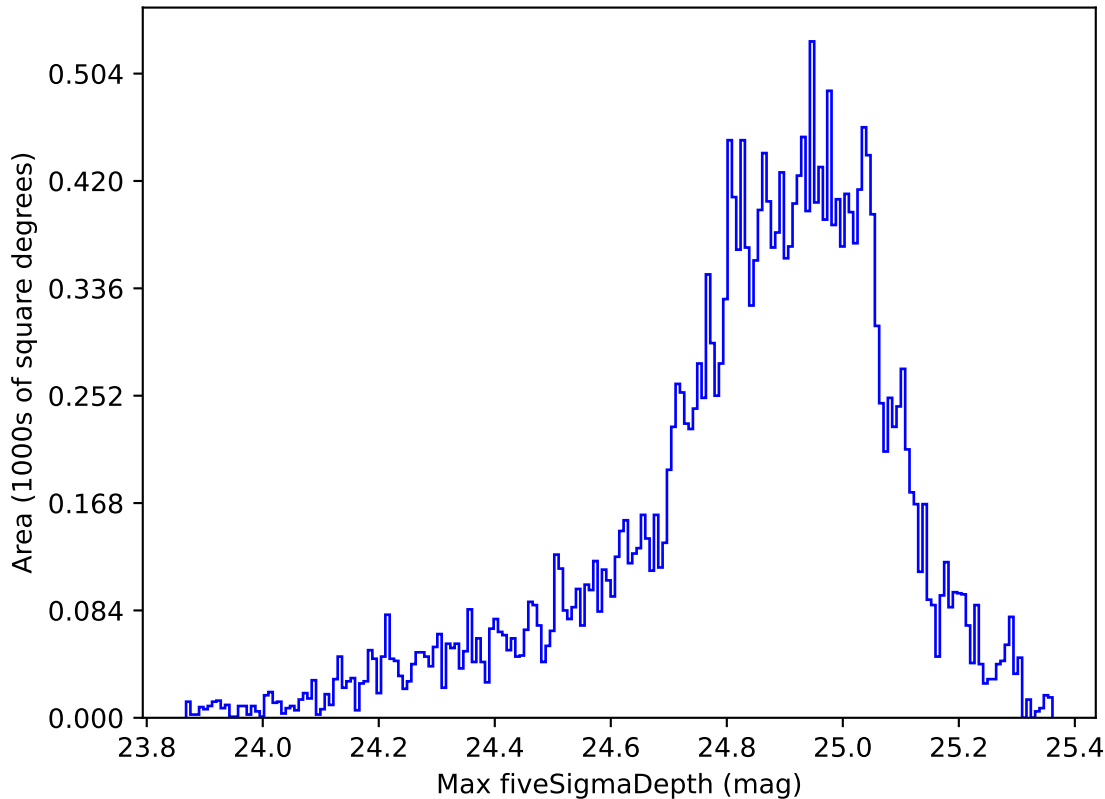
weather_cloudso8v3.4_10yrs Yr 1 all bands: Max fiveSigmaDepth
