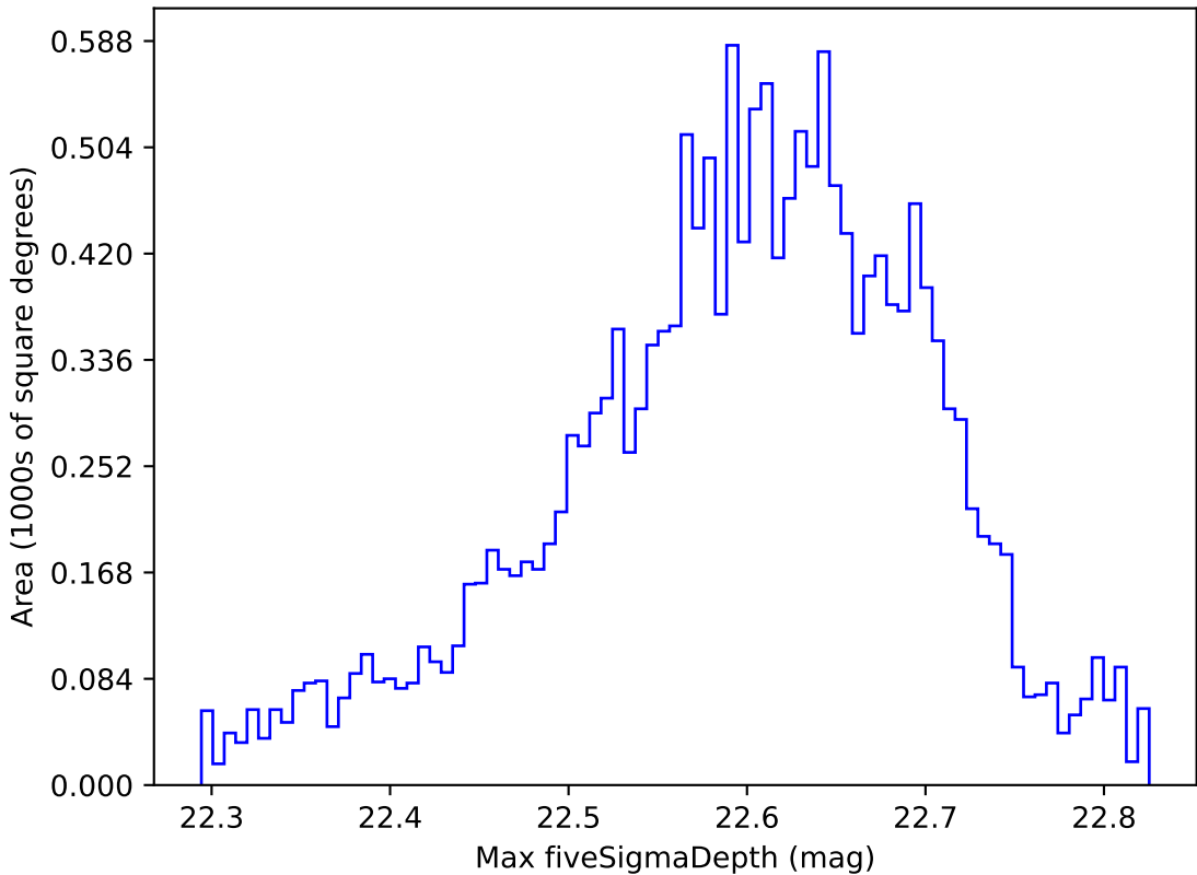
weather_cloudso8v3.4_10yrs WFD y band: Max fiveSigmaDepth
