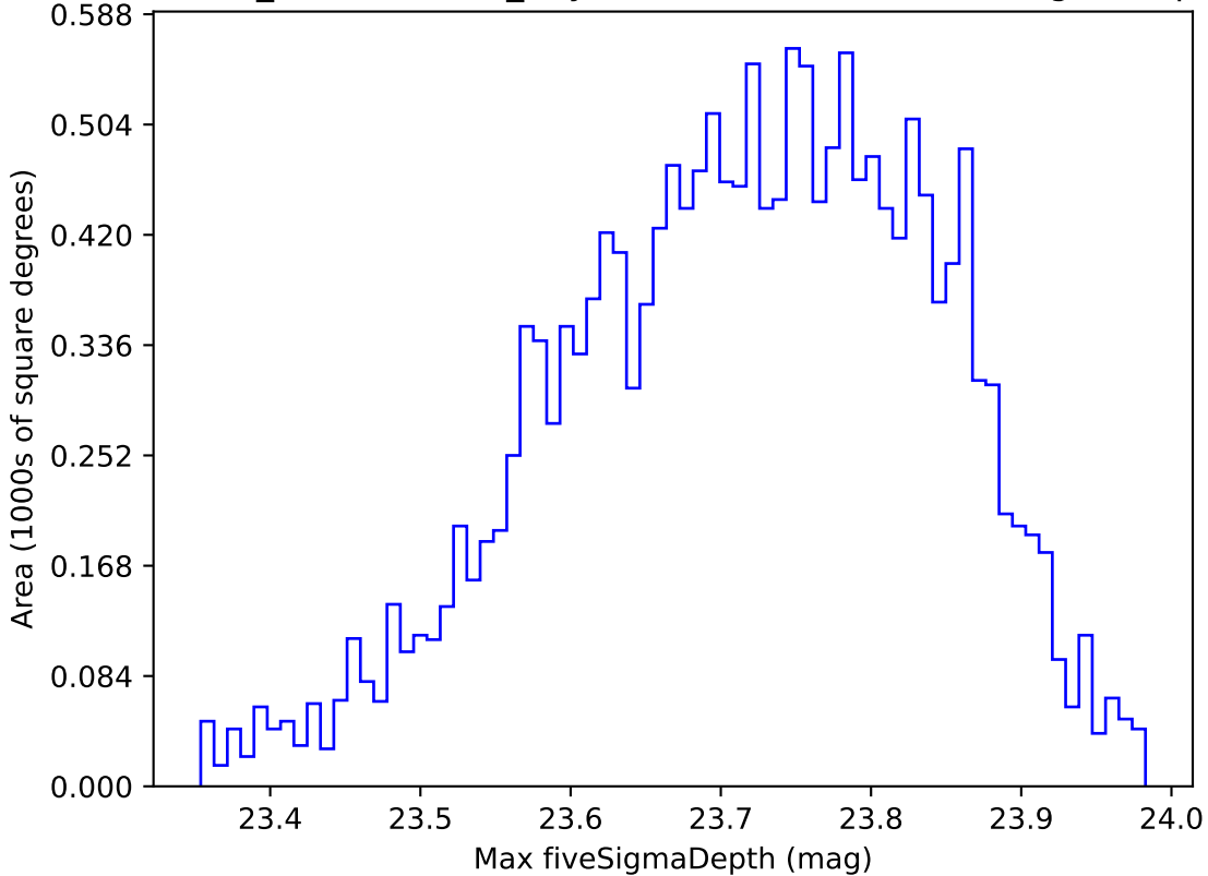
weather_cloudso8v3.4_10yrs WFD u band: Max fiveSigmaDepth
