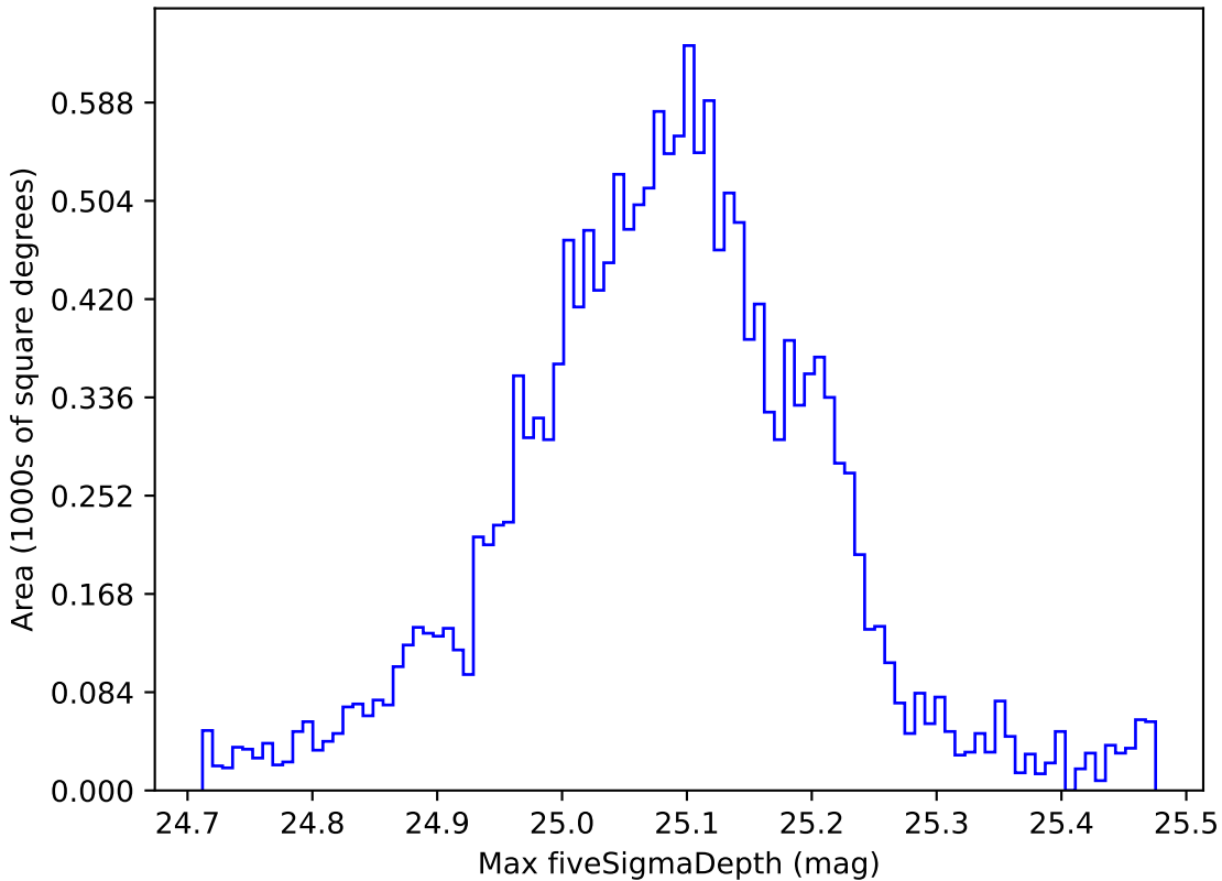
weather_cloudso8v3.4_10yrs WFD g band: Max fiveSigmaDepth
