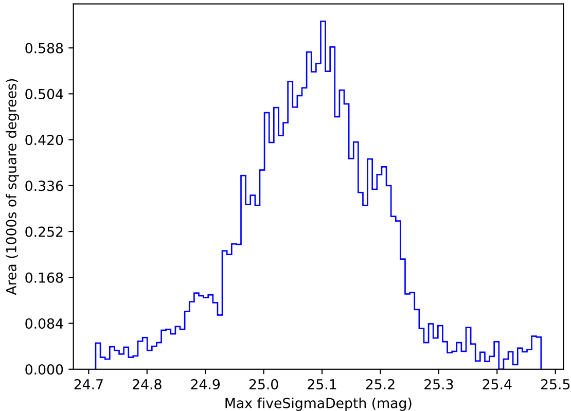
weather_cloudso8v3.4_10yrs WFD all bands: Max fiveSigmaDepth
