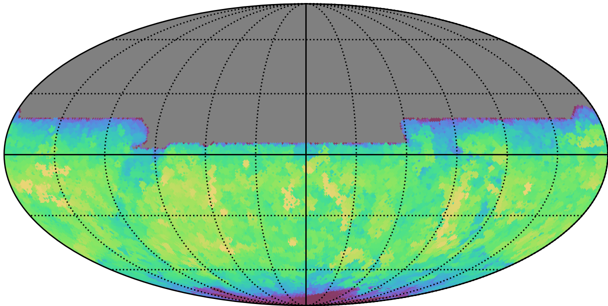
weather_cloudso8v3.4_10yrs All sky y band: Max fiveSigmaDepth
