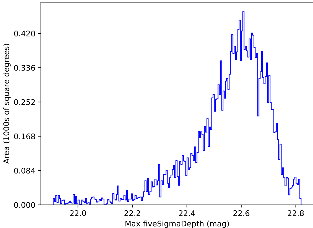
weather_cloudso8v3.4_10yrs All sky y band: Max fiveSigmaDepth
