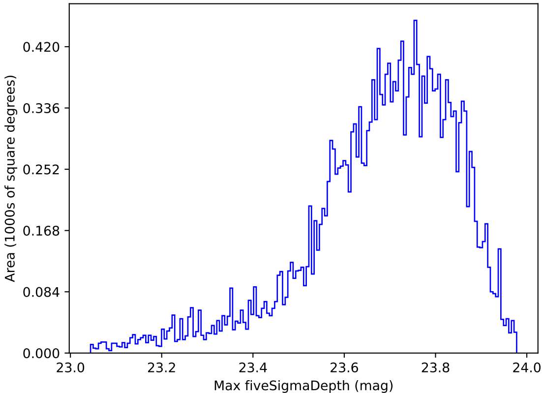
weather_cloudso8v3.4_10yrs All sky u band: Max fiveSigmaDepth
