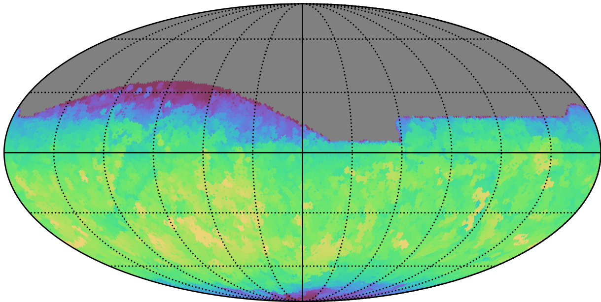
weather_cloudso8v3.4_10yrs All sky r band: Max fiveSigmaDepth
