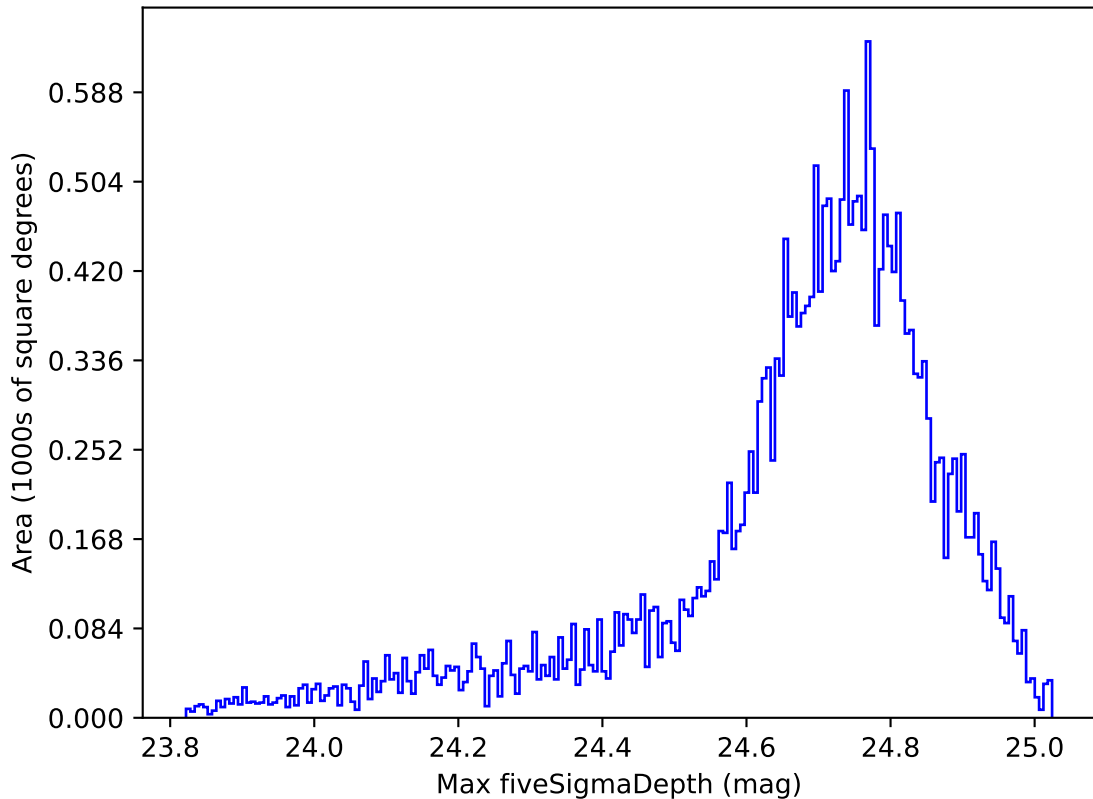
weather_cloudso8v3.4_10yrs All sky r band: Max fiveSigmaDepth
