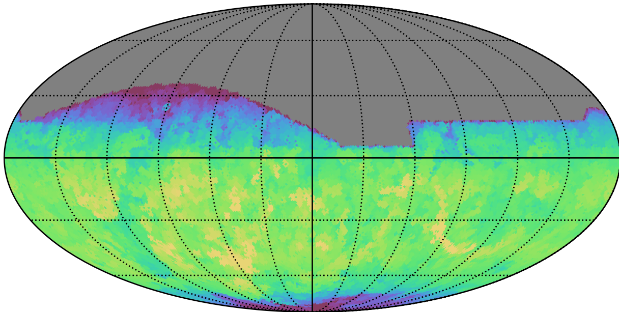
weather_cloudso8v3.4_10yrs All sky i band: Max fiveSigmaDepth
